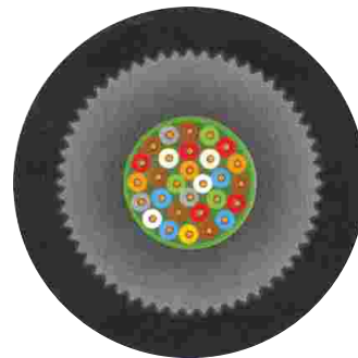
Cross section of a Polyethylene duct with ribbed interior surface for fibre optic cable
